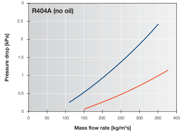
Pressure drop
