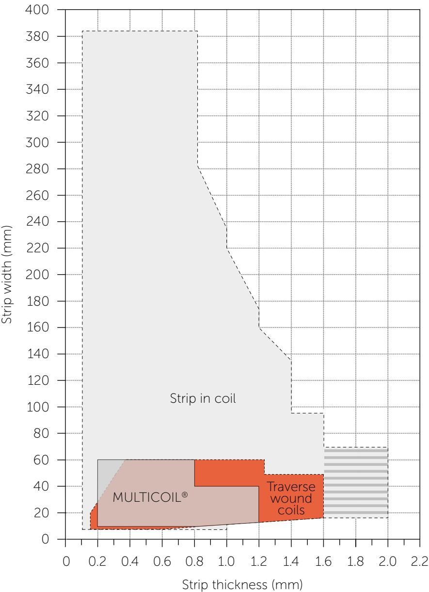
Fig. 4: Ranges of available dimensions for hot-dip tinned strip. For some base materials there may be restrictions.
