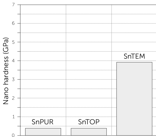
Fig. 3: Nano hardness of the top layer of the different hot-dip tin coating types, measured by nanoindentation. Nano hardness is independent of the coating thickness.
