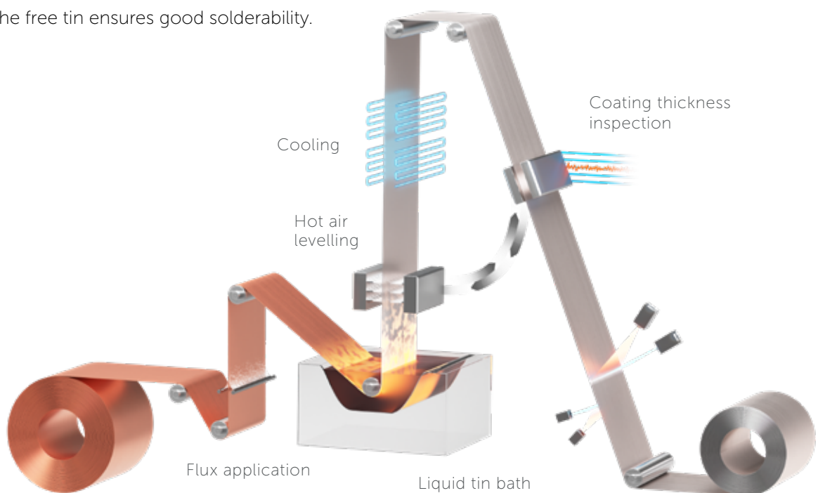
Fig. 1: Schematic of hot-dip tinning process
