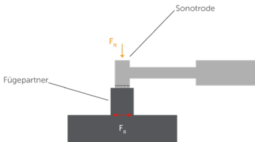
Figure 11 – Principle of ultrasonic welding
