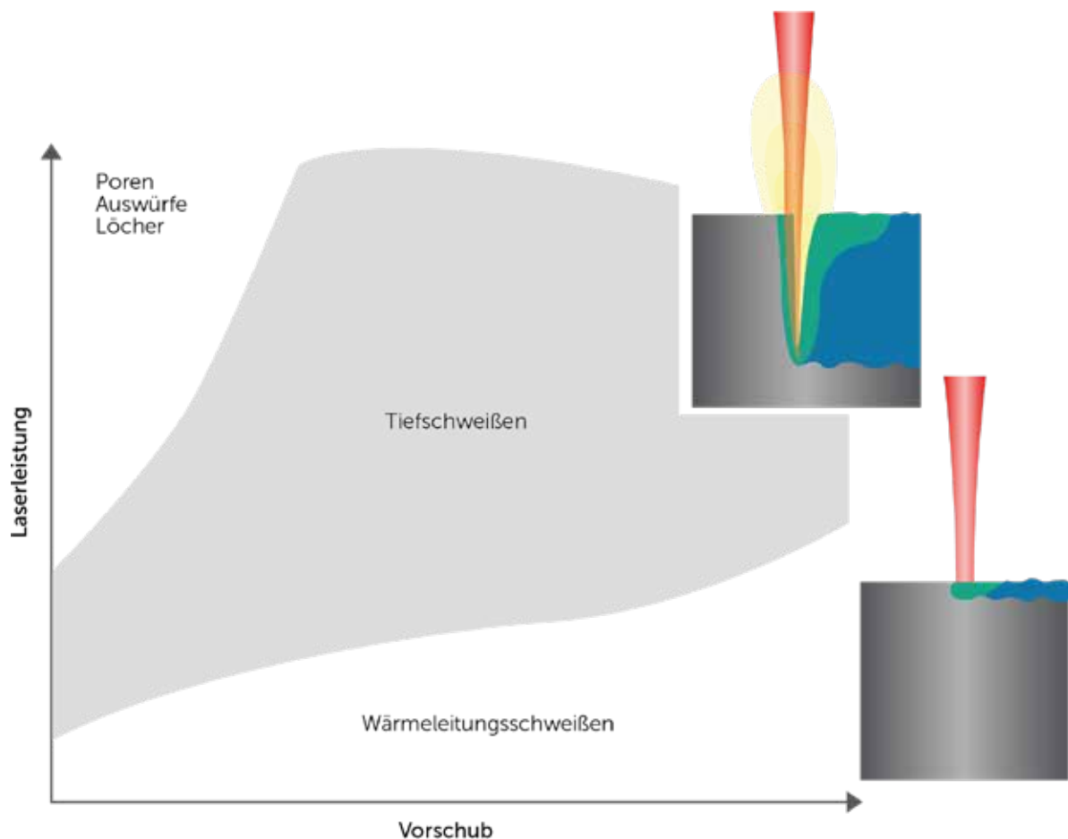
Figure 7 – Process window for cw laser beam welding
