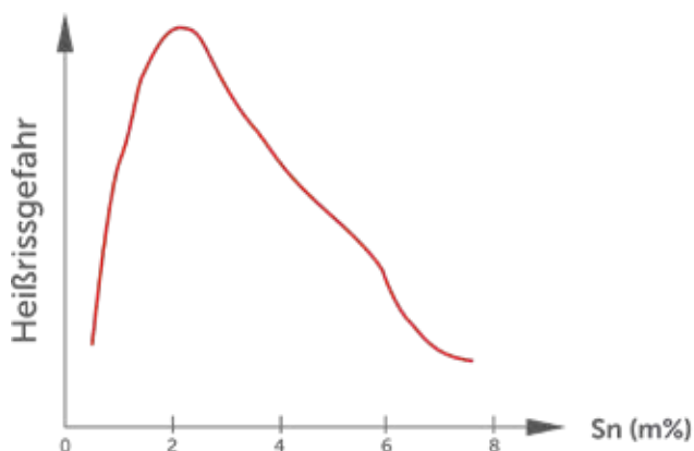
Figure 18 – Qualitative correlation between the tin content in a bronze and the risk of hot cracking during fusion welding
