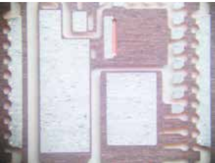
Inhomogeneous plated surface
