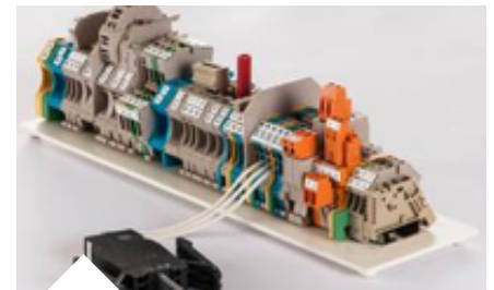
Terminal blocks contain springs made of high-performance alloys, such as Wieland-K55 R800
